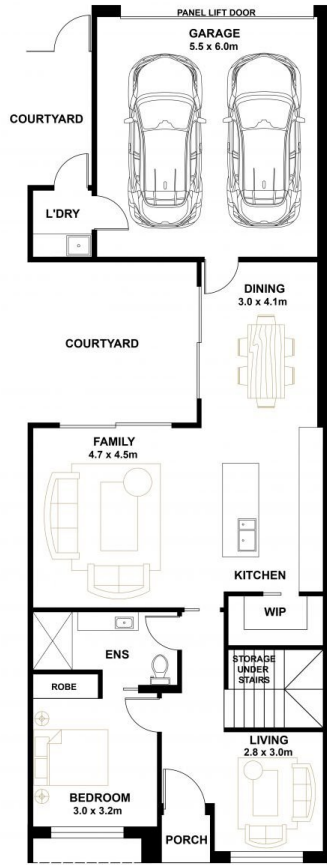
LOWER FLOOR
