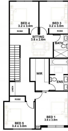
UPPER FLOOR
