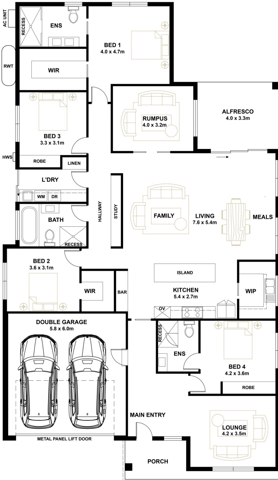
FLOOR PLAN
