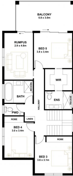
UPPER FLOOR PLAN
