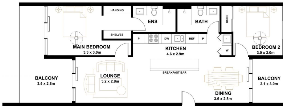
FLOOR PLAN
