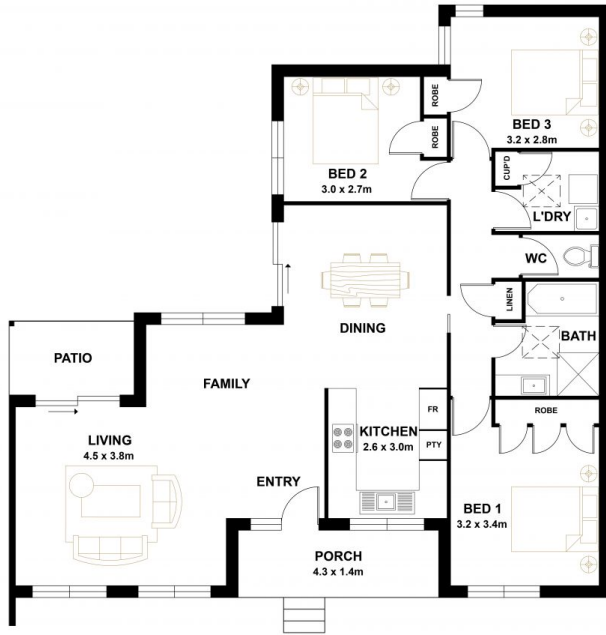
FLOOR PLAN
